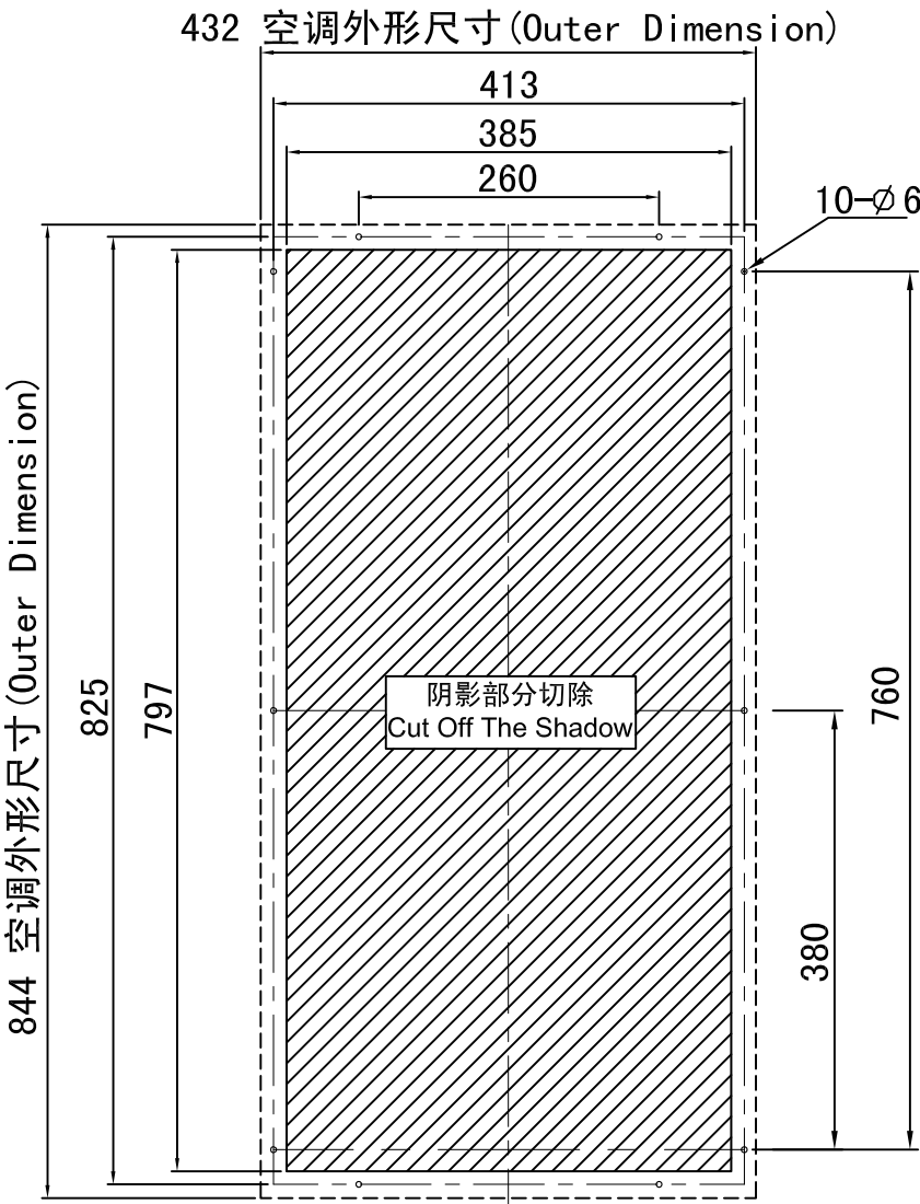
柜门开孔尺寸/Cabinet Door Cutting Dimension
