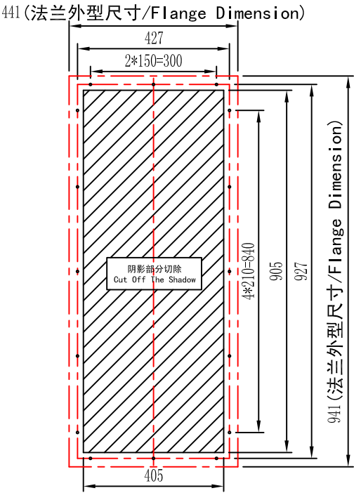
图1-柜门开孔尺寸 Figure 1-Cabinet Door Cutting Dimension
