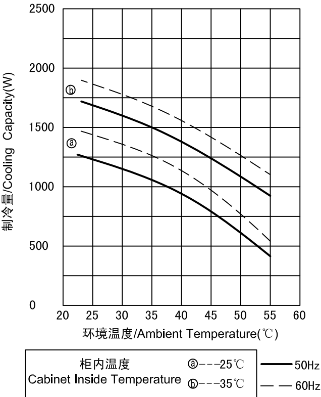
冷量曲线/Cooling Capacity Chart
