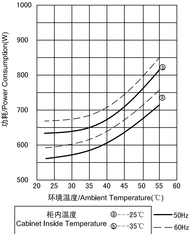
功耗曲线/Power Consumption Chart
